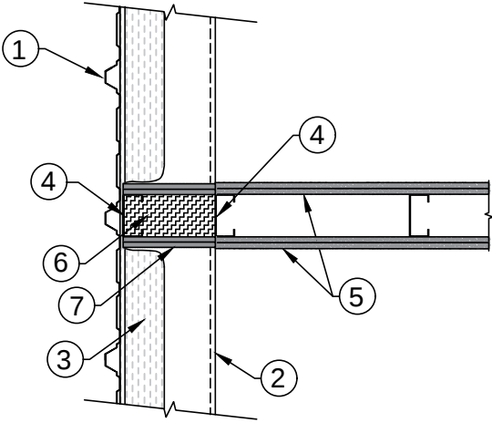
Section A-A 2-Hour Rated Interior Wall
