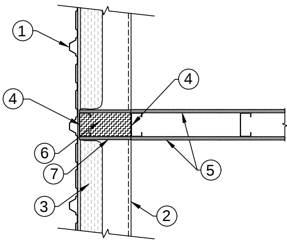
Section A-A 1-Hour Rated Interior Wall
