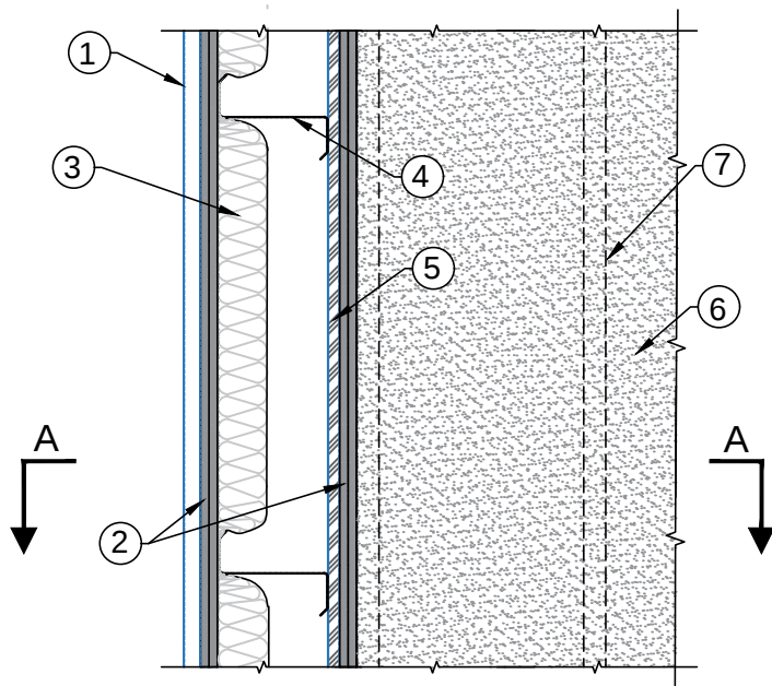
2-Hour Rated Interior Wall to 2-Hour Rated Exterior Wall (UL V421 or equivalent)
