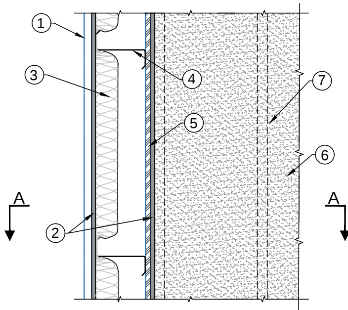
1-Hour Rated Interior Wall to 1-Hour Rated Exterior Wall (UL V421 or equivalent)
