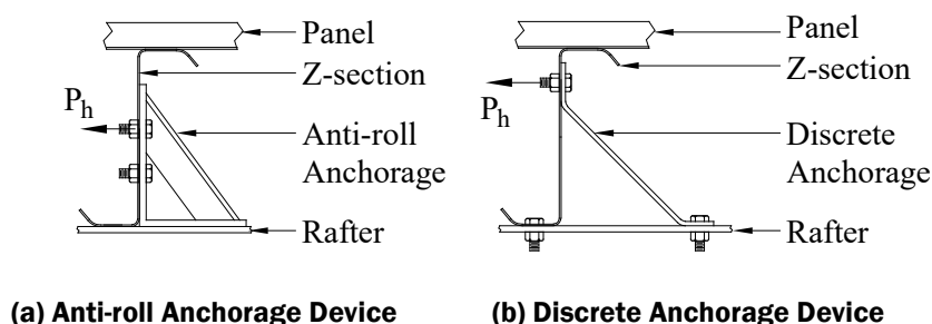
Figure 5.5-9 Support Anchorage Configurations
