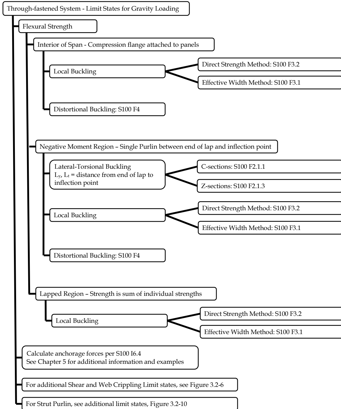
Figure 3.2-1 Through-Fastened System - Limit States for Gravity Loading
