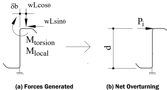
Figure 5.5-1 Free Body Diagram of Forces Generated
