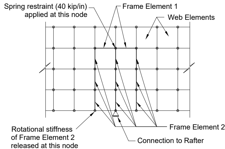
Figure 5.5.6-5 Frame Elements to Represent Anti-roll Anchorage
