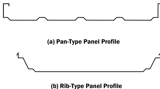
Figure 1.1-2 Panel Profiles
