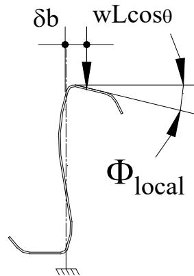
Figure 5.5-7 Local Deformation of Z-Section
