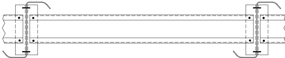
Figure 3.3-7 Third Point Discrete Braces
