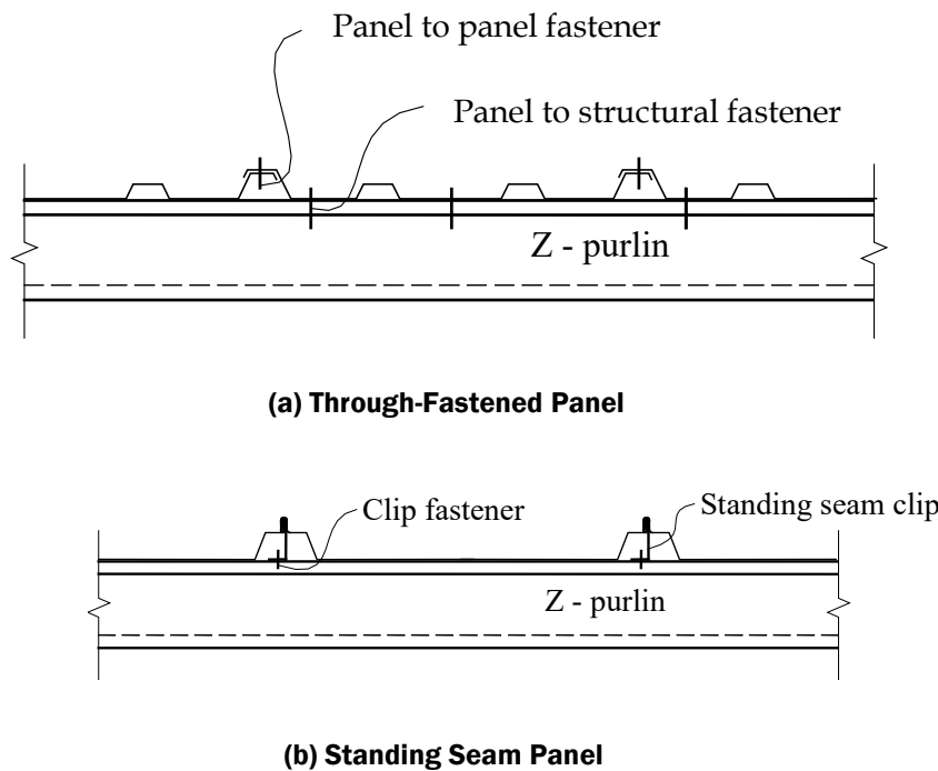
Figure 1.1-1 Roof Panel Profiles
