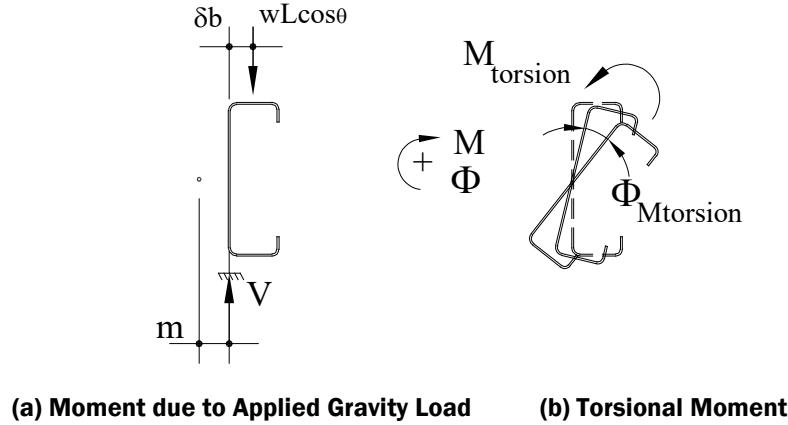
Figure 5.5-6 Moments Acting on C-Section
