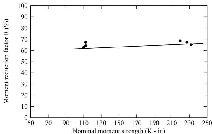
Figure 2.3-4 Reduction Factor versus Nominal Moment Strength
