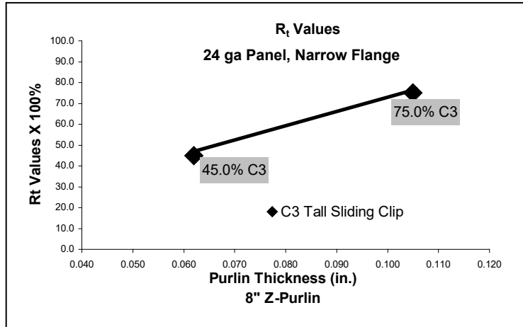
Figure 2.3.14 Determination of Panel Thickness Trend
