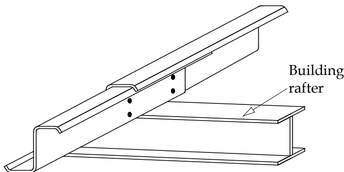
(b) Lapped Z-Purlins
