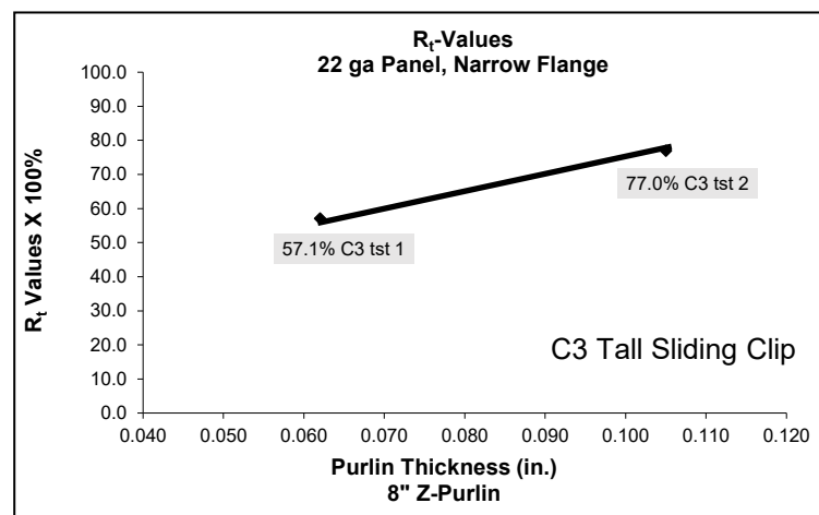
Figure 2.3-9 Initial test with Assumed Controlling Clip Type
