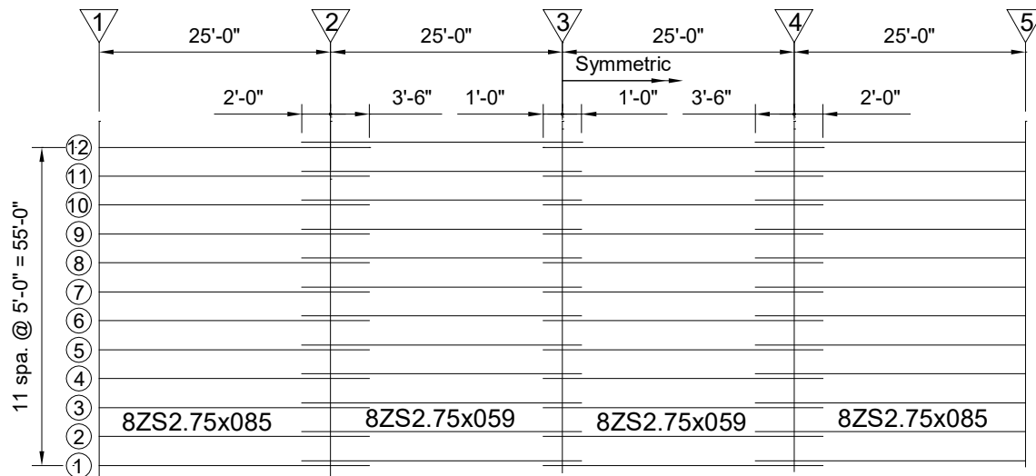
Figure 5.5.6-2 Roof Layout for Finite Element Model
