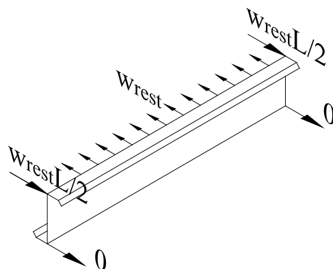
Figure 5.5-4 Uniform Restraint Force in Panels
