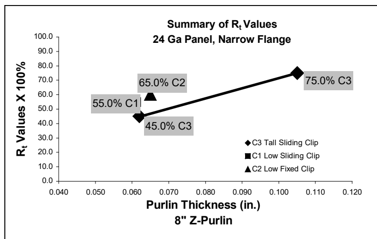
Figure 2.3-15 Controlling Clip Type Verification
