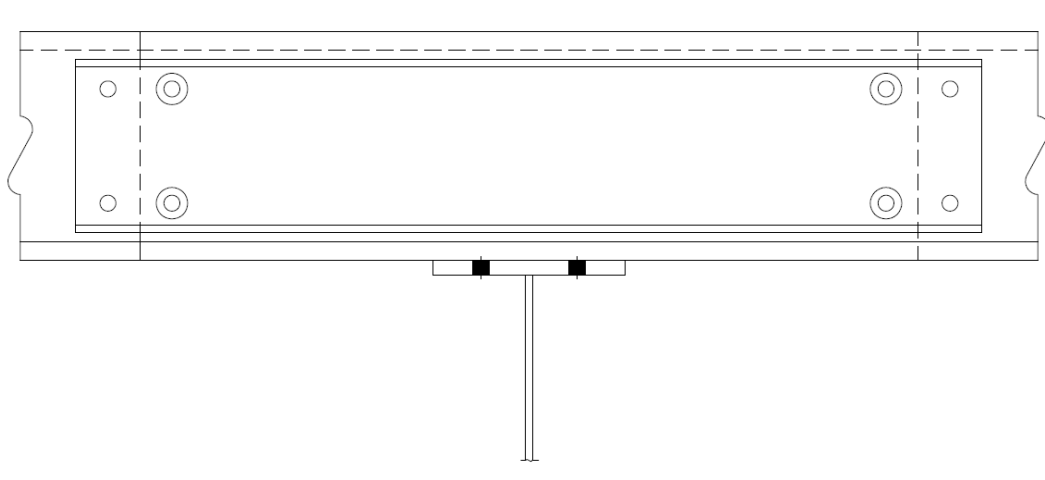
Figure 25: Channel Reinforcement for Continuous Purlins
