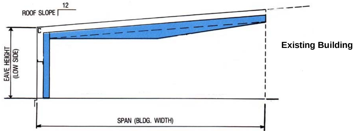
Figure 4: Lean-To Frame
