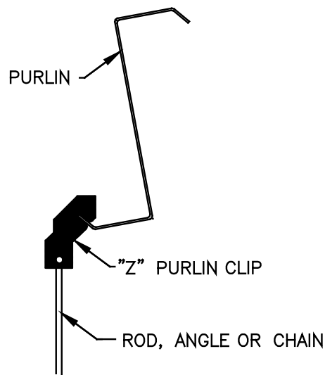
Figure 22: Incorrect Way to Hang Loads on Purlin
