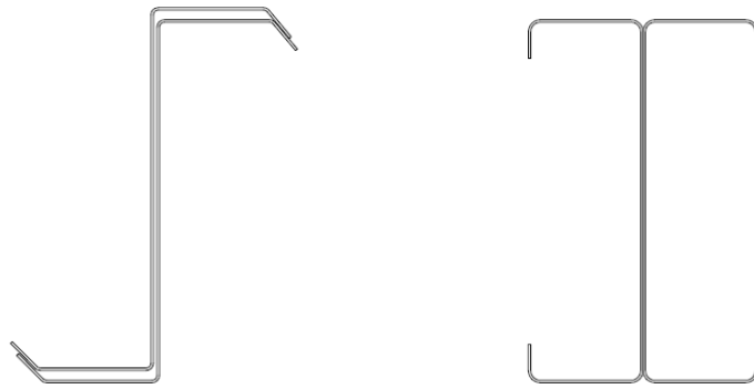
Figure 6: Nested Z Shapes and Back to Back C Shapes for Laps
