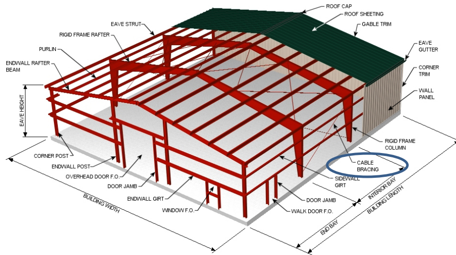
Figure 10: Typical X-Bracing for Longitudinal Lateral Loads
